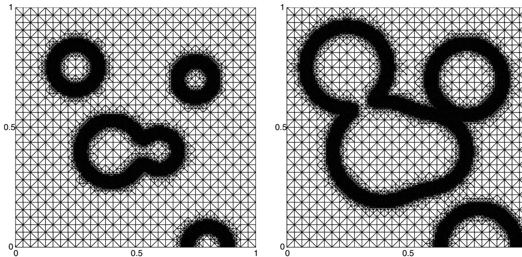
Figure 7.3. Diffuse interfaces with topological change.
