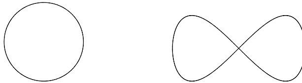
Figure 1.2. A lemniscate, parametrized over the unit circle.
