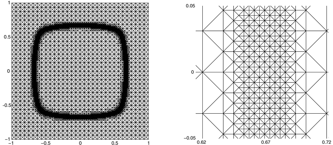
Figure 7.1. Meshes.
